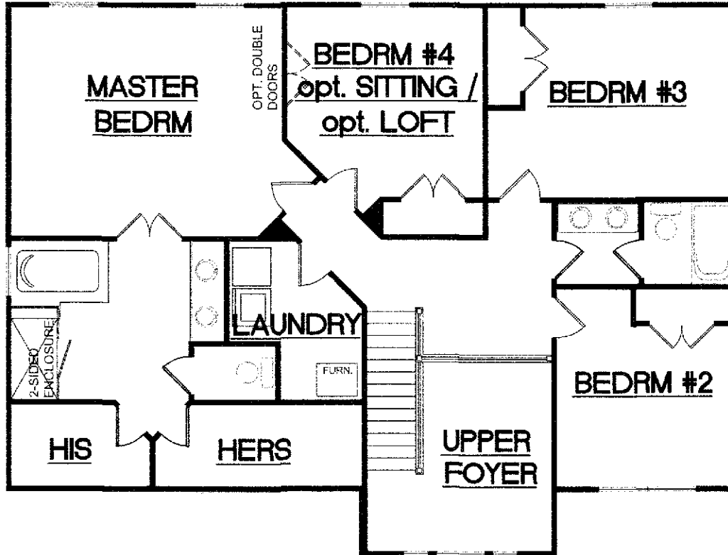
WASHINGTON - SECOND FLOOR PLAN
